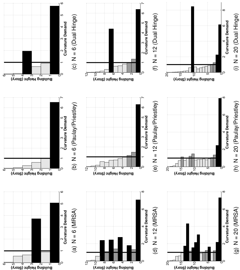
Figure 7.9: Curvature Demand Profiles for Alternate Detailing Methods
