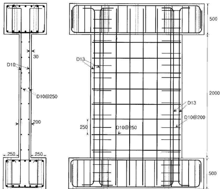
Figure A.20: Oh et al. Specimen Geometry (Oh et al., 2002)
