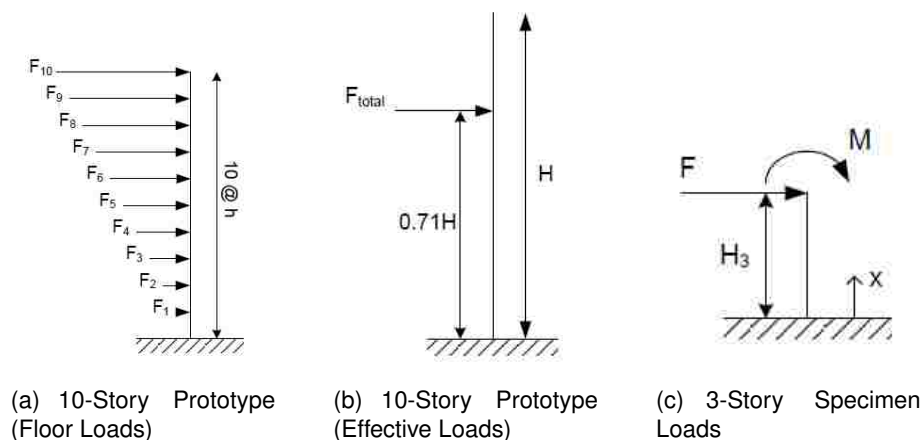
Figure A.24: UW1 Load Pattern
