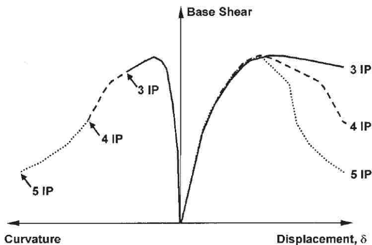
Figure 3.2: Softening Cantilever Wall Behavior (Coleman and Spacone, 2001)
