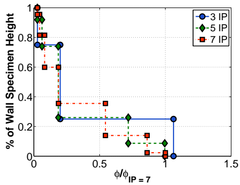
(a) \phi Diagram ( \Delta = 0.30\% )
