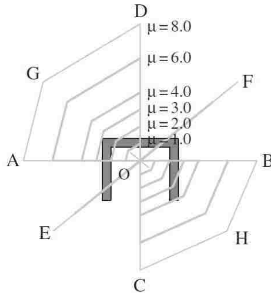
Figure A.30: TUA/TUB Loading Protocol (Beyer et al, 2007)
